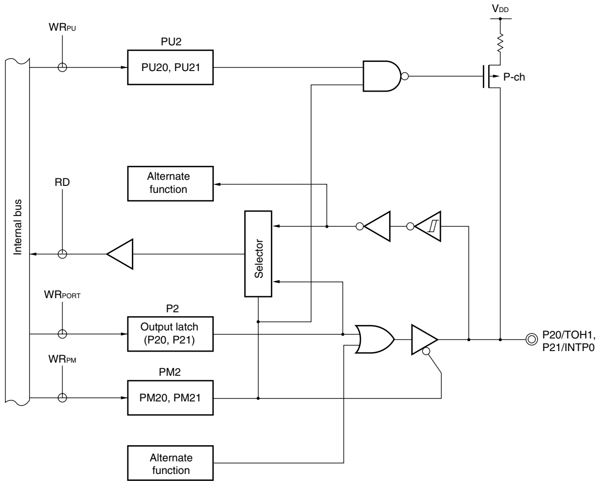
Figure 4-5. Block Diagram of P20 and P21 ( \mu PD78F950x)
