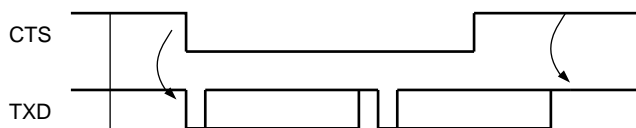
Figure 21-28. Transmitter Behavior when Operating with Hardware Handshaking
