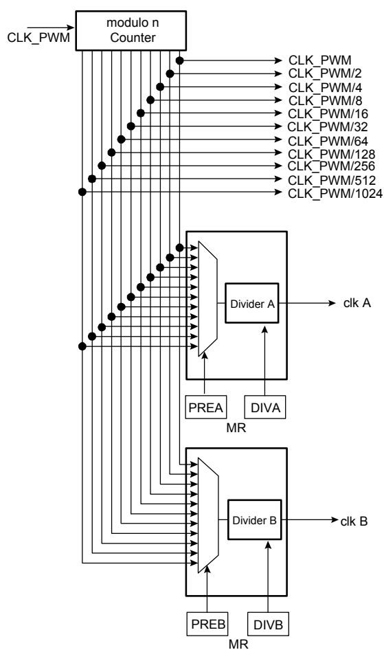
Figure 24-2. Functional View of the Clock Generator Block Diagram
