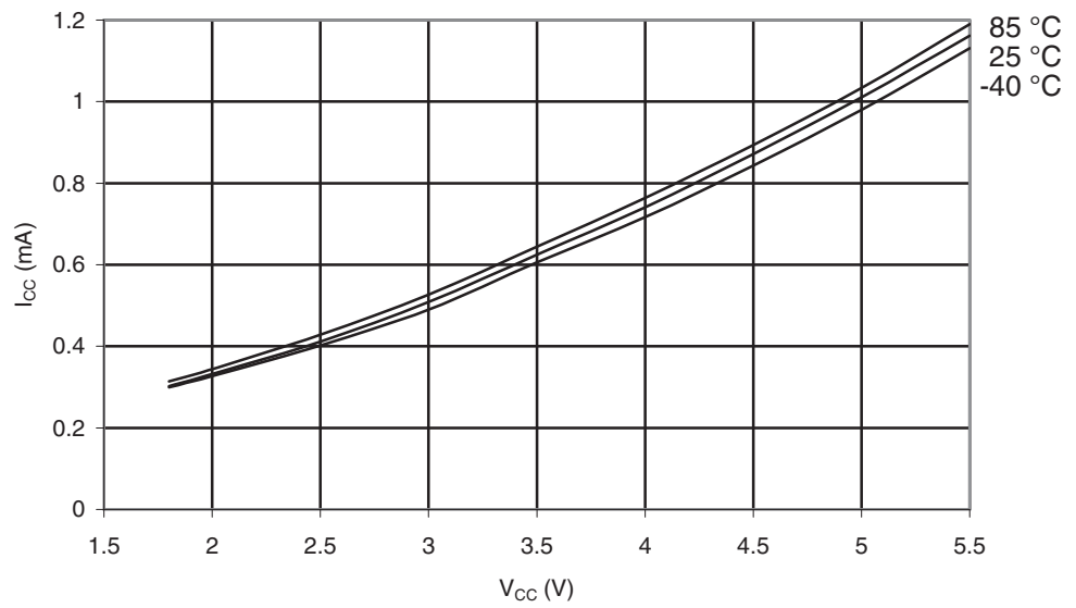
Figure 28-4. ATmega164A: Active Supply Current vs. V_{CC} (Internal RC Oscillator, 1 MHz).
