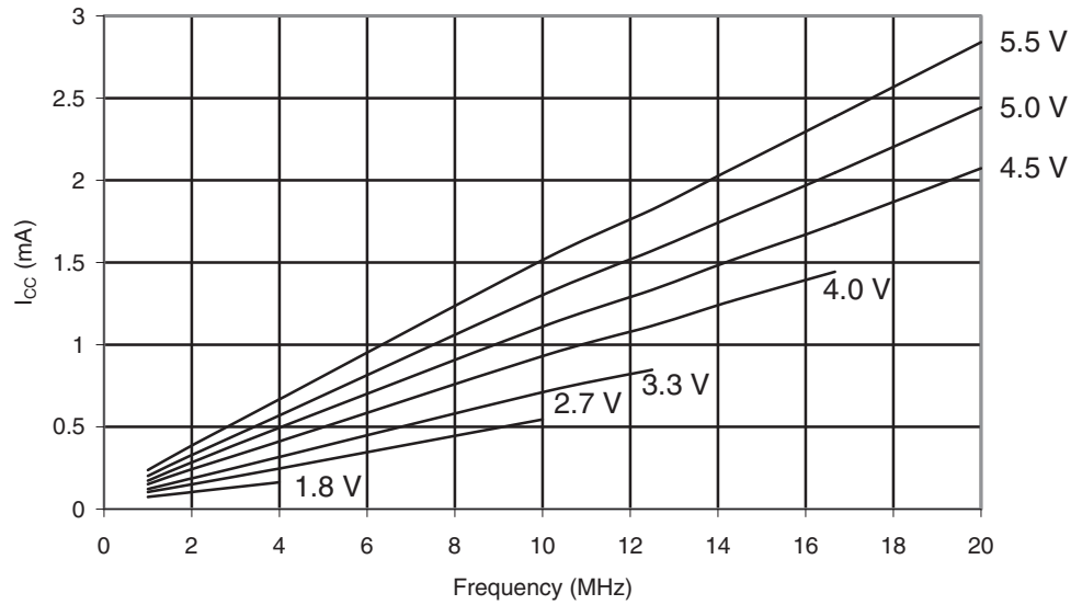
Figure 28-301. ATmega1284: Idle Supply Current vs. Frequency (1 - 20 MHz)
