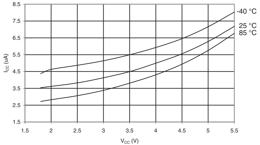
Figure 28-391. ATmega1284P: Watchdog Timer Current vs. V_{CC}
