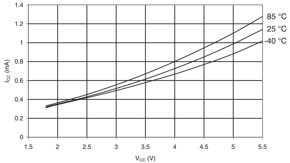
Figure 28-302. ATmega1284: Idle Supply Current vs. V_{CC} (Internal RC Oscillator, 8 MHz)
