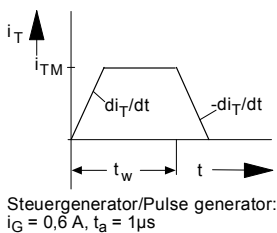
Diagram for the determination of the total energy W_{tot} for a trapezoidal current pulse for one arm at: given rate of rise of on-state current di_T/dt , forward off-state voltage v_{DM} \leq 0,67 V_{DRM} , maximum reverse voltage v_{RM} \leq 50 V , rate of rise of off-state voltage dv_R/dt \leq 100 V/\mu s .
