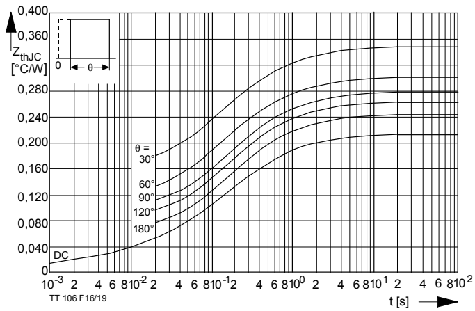
Bild / Fig. 18 Transienter innerer Wärmewiderstand je Zweig Z_{thJC} . Transient thermal impedance, junction to case, per arm Z_{thJC} .
