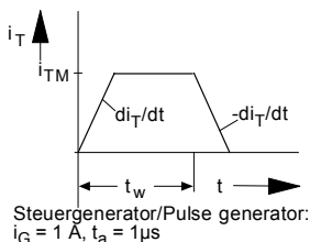
Diagram for the determination of the total energy W_{tot} for a trapezoidal current pulse for one arm at: given rate of rise of on-state current di_T/dt , forward off-state voltage v_{DM} \leq 0,67 V_{DRM} , maximum reverse voltage v_{RM} \leq 50 V , rate of rise of off-state voltage dv_R/dt \leq 100 V/\mu s .
