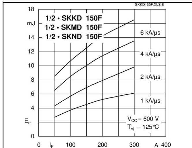
Fig. 6 Typ. turn-off energy dissipation per pulse
