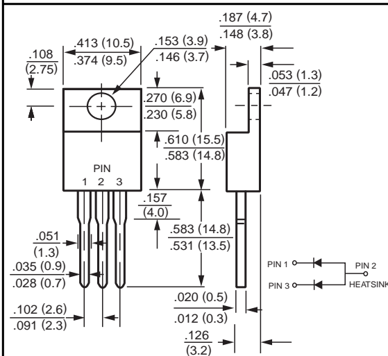
TO-220
