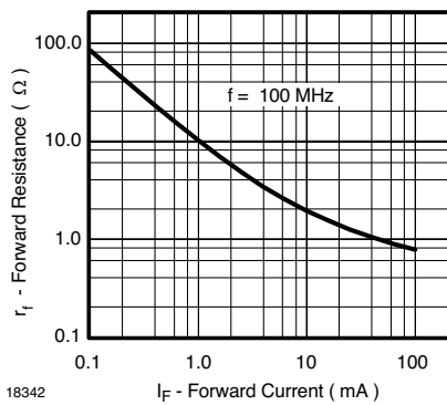
Fig. 1 Forward Resistance vs. Forward Current
