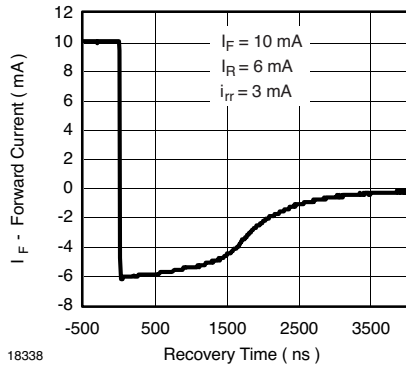
Fig. 5 Typical Charge Recovery Curve
