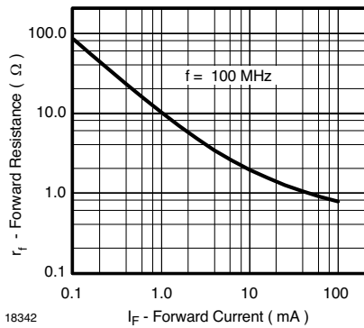
Fig. 1 Forward Resistance vs. Forward Current
