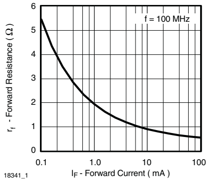
Figure 1. Forward Resistance vs. Forward Current
