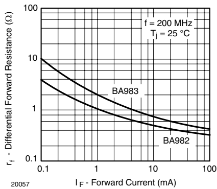
Figure 1. Differential Forward Resistance vs. Forward Current
