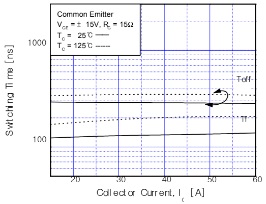
Fig 11. Turn-Off Characteristics vs. Collector Current
