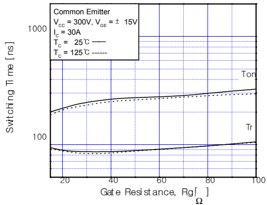
Fig 7. Turn-On Characteristics vs. Gate Resistance
