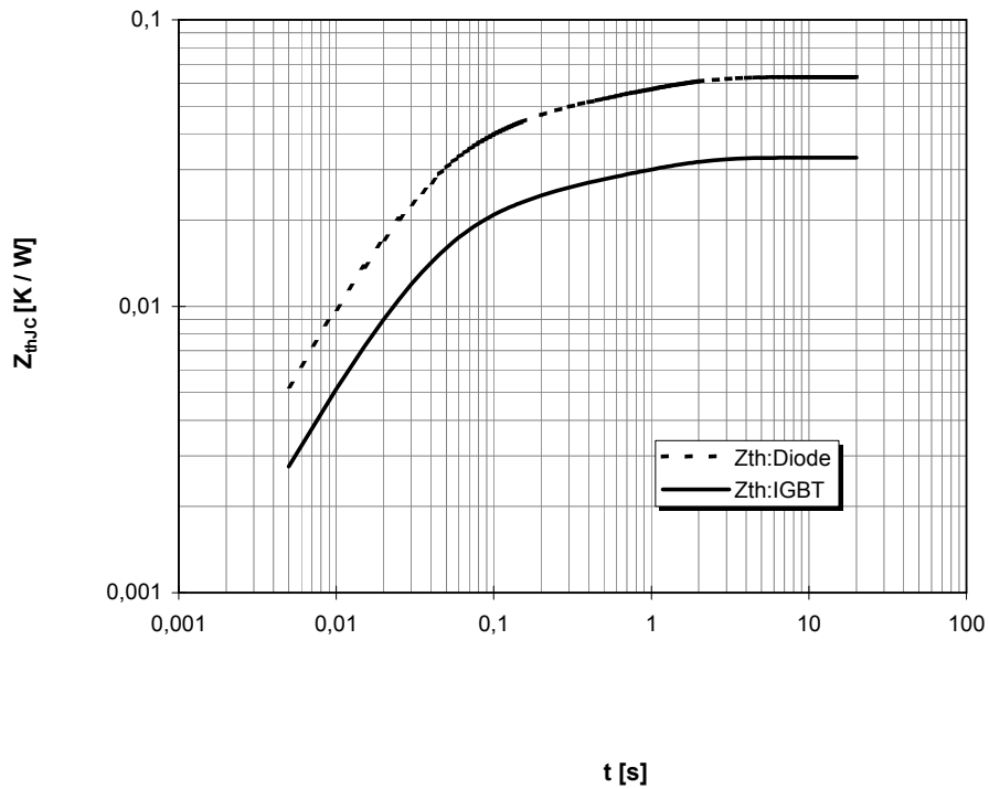
Transienter Wärmewiderstand Z_{thJC} = f(t) Transient thermal impedance
