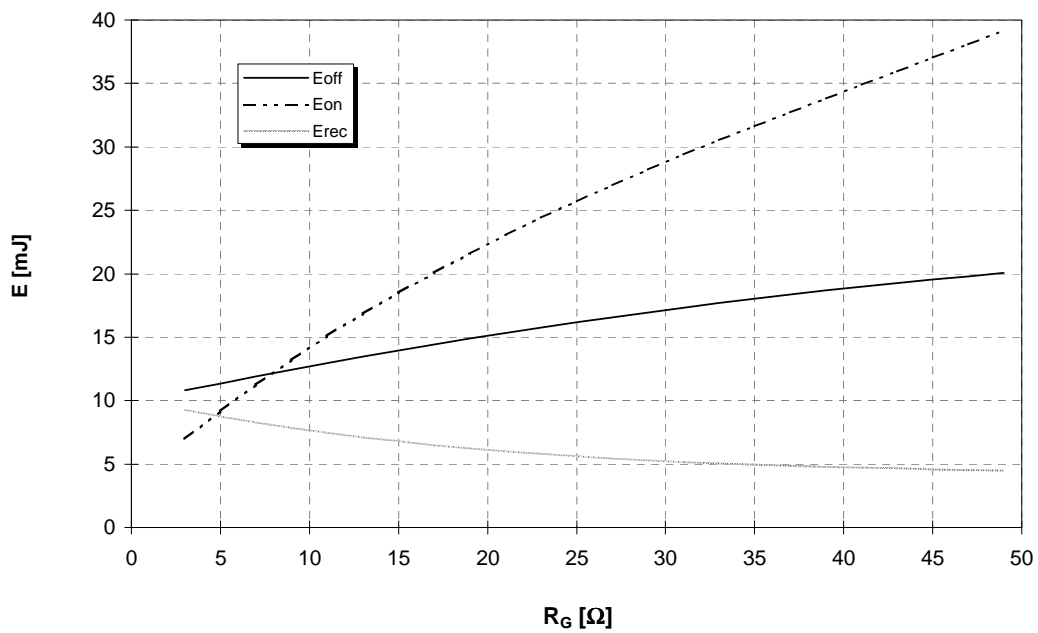
Schaltverluste (typisch) E_{on} = f(R_G) , E_{off} = f(R_G) , E_{rec} = f(R_G) Switching losses (typical) V_{GE}=15V , I_c = 100A , V_{CE} = 600V , T_j = 125^\circ C
