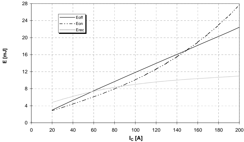
Schaltverluste (typisch) E_{on} = f(I_c) , E_{off} = f(I_c) , E_{rec} = f(I_c) Switching losses (typical) V_{GE}=15V , R_{gon} = R_{goff} = 5,6 \Omega , V_{CE} = 600V , T_j = 125^\circ C
