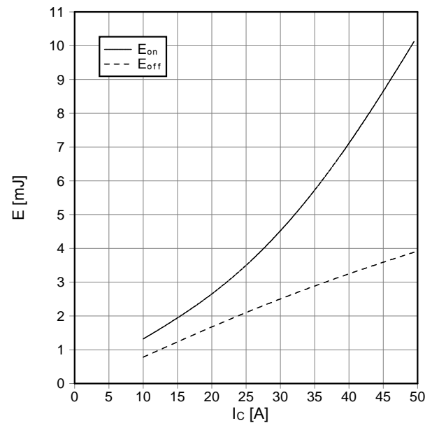
Schaltverluste IGBT-Wechselr. (typisch) switching losses IGBT-inverter (typical) E_{on} = f(I_c) , E_{off} = f(I_c) V_{GE} = \pm 15\text{ V} , R_{Gon} = 36\ \Omega , R_{Goff} = 36\ \Omega , V_{CE} = 600\text{ V} , T_{vj} = 125^\circ\text{C}
