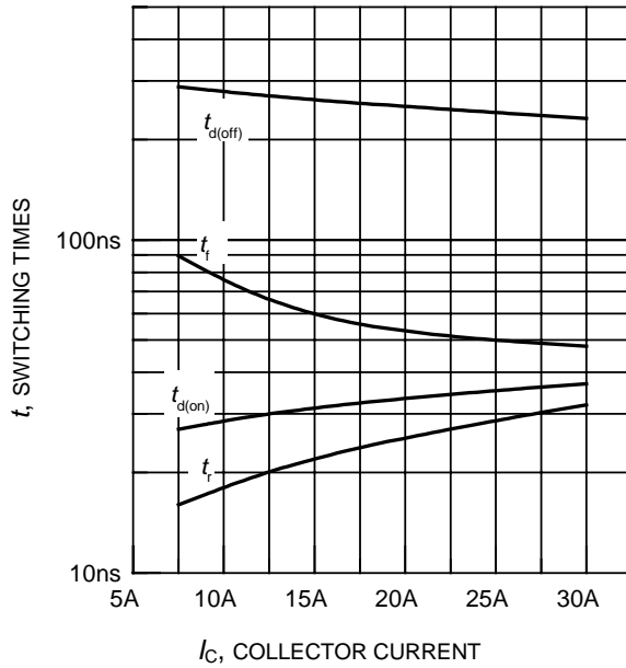
Figure 9. Typical switching times as a function of collector current (inductive load, T_j = 150^\circ\text{C} , V_{CE} = 400\text{V} , V_{GE} = 0/+15\text{V} , R_G = 21\ \Omega , Dynamic test circuit in Figure E)
