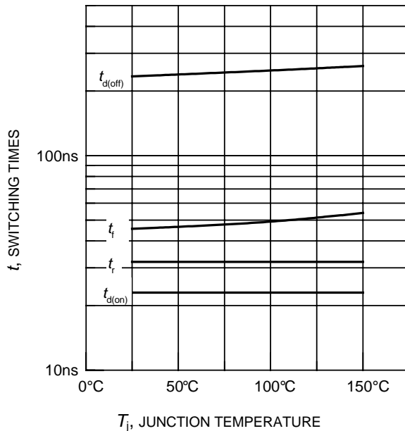
Figure 11. Typical switching times as a function of junction temperature (inductive load, V_{CE} = 400\text{V} , V_{GE} = 0/+15\text{V} , I_C = 15\text{A} , R_G = 21\ \Omega , Dynamic test circuit in Figure E)
