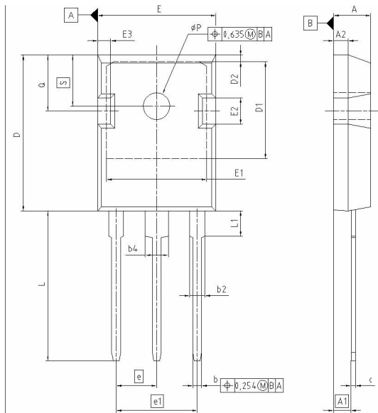
PG-TO247-3-21
