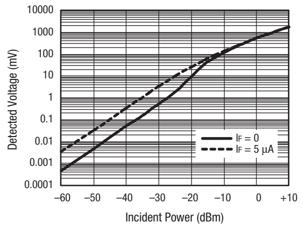
Figure 3. Detector Voltage @ 2.45 GHz (100 k \Omega Video Resistance)
