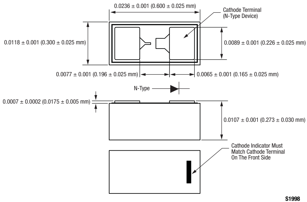
Figure 5. SMS7621-060 Package Dimension Drawing
