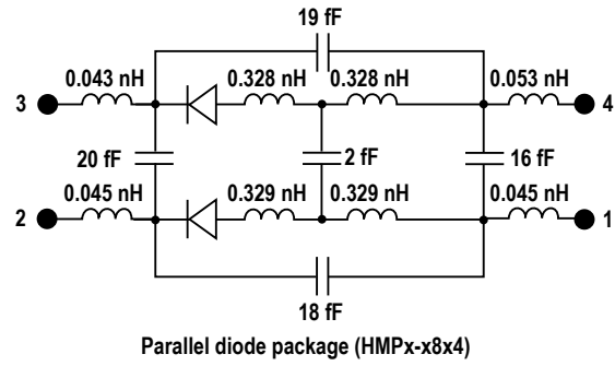
Figure 16b. Linear Equivalent Circuit of the Minipak QFN PIN Diode
