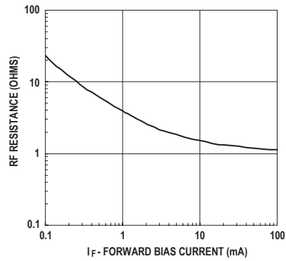
Figure 6. Total RF Resistance at 25^\circ\text{C} vs. Forward Bias Current
