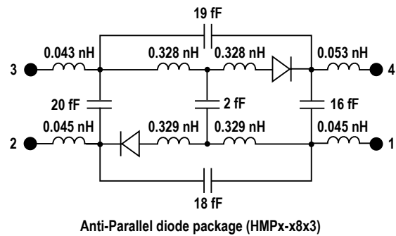
Anti-Parallel diode package (HMPx-x8x3)
