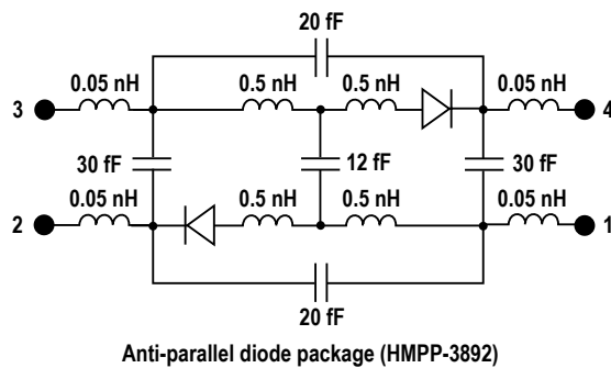
Anti-parallel diode package (HMPP-3892)
