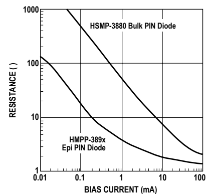
Figure 15. Resistance vs. Forward Bias.
