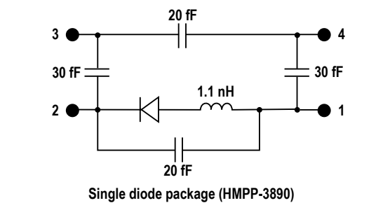
Single diode package (HMPP-3890)
