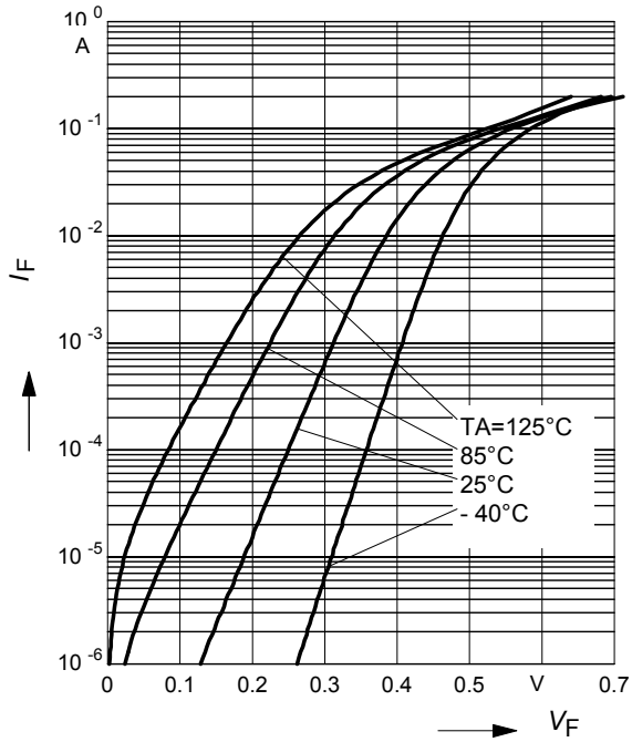
Forward current I_F = f(V_F) (per diode)
