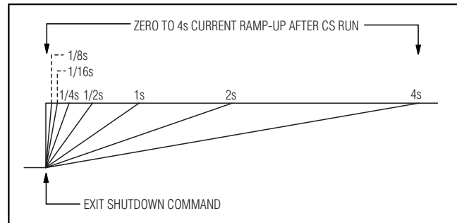
Figure 4. Ramp-Up Behavior
