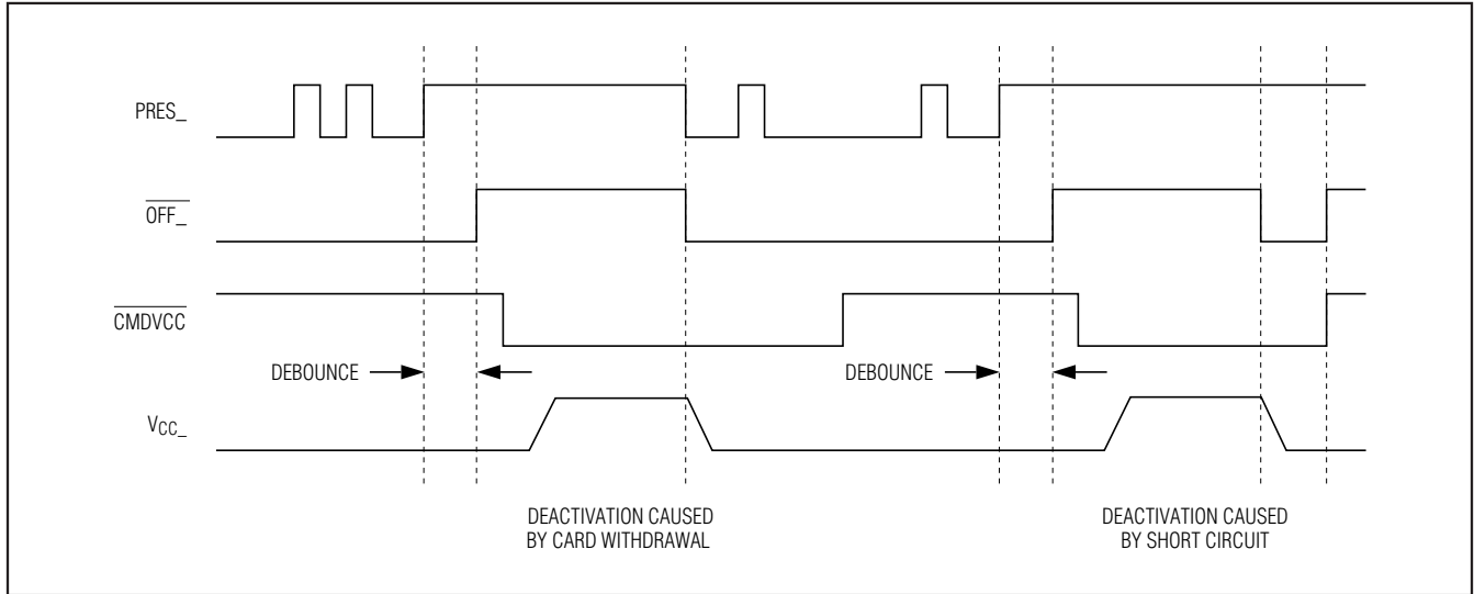
Figure 6. Behavior of PRES_ , \overline{OFF}_ , \overline{CMDVCC} , and VCC_
