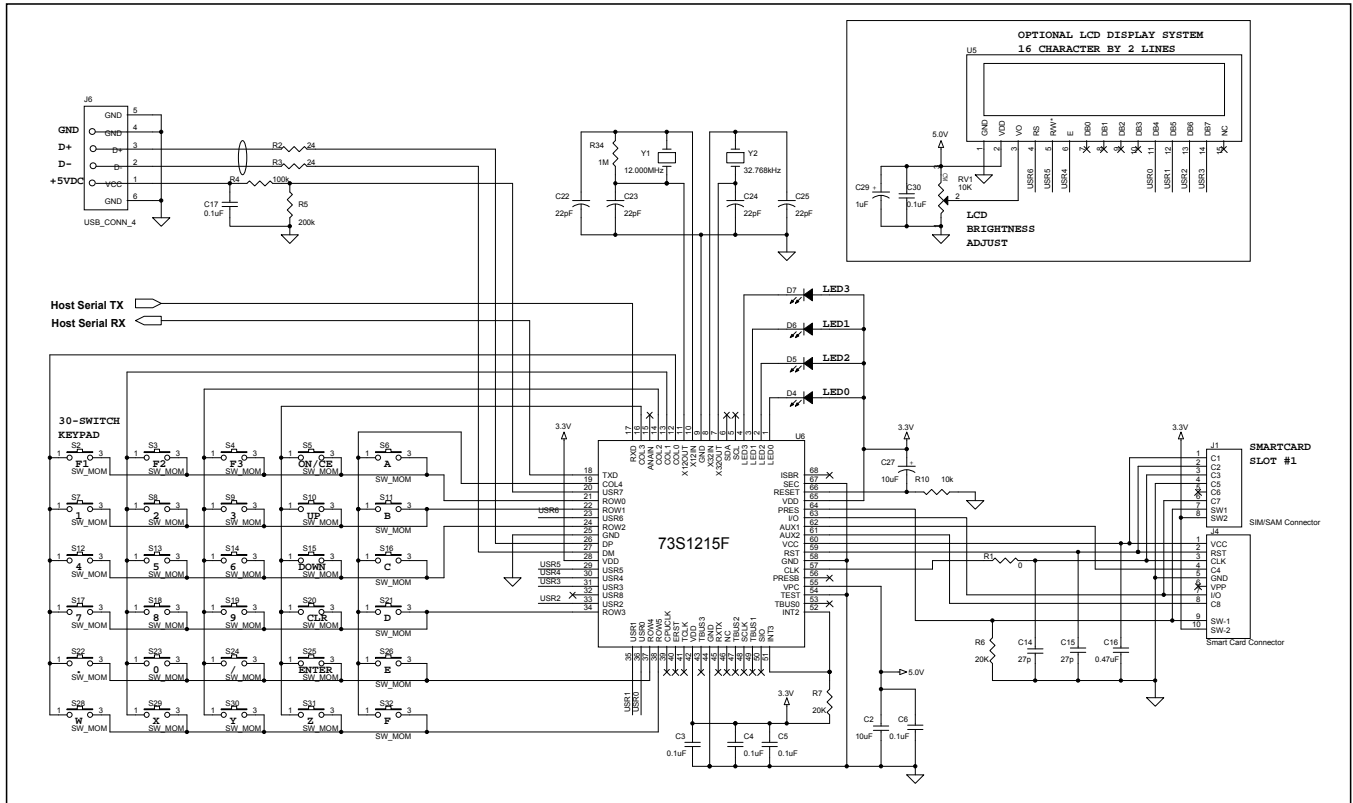
Figure 26: 73S1215F Typical Application Schematic
