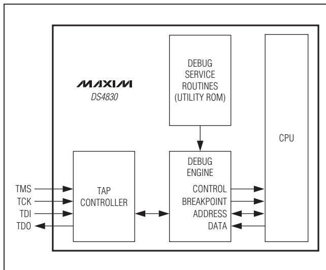
Figure 10. In-Circuit Debugger
