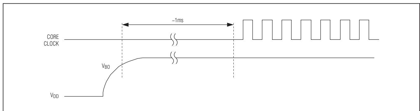
Figure 8. System Timing
