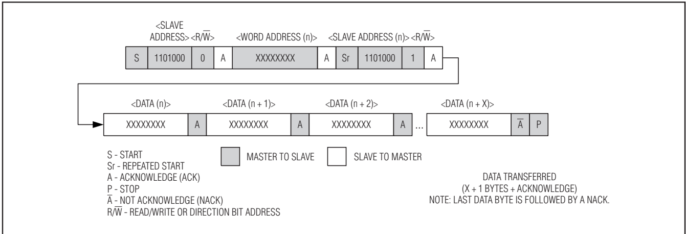
Figure 6. Data Write/Read (Write Pointer, Then Read)—Slave Receive and Transmit
