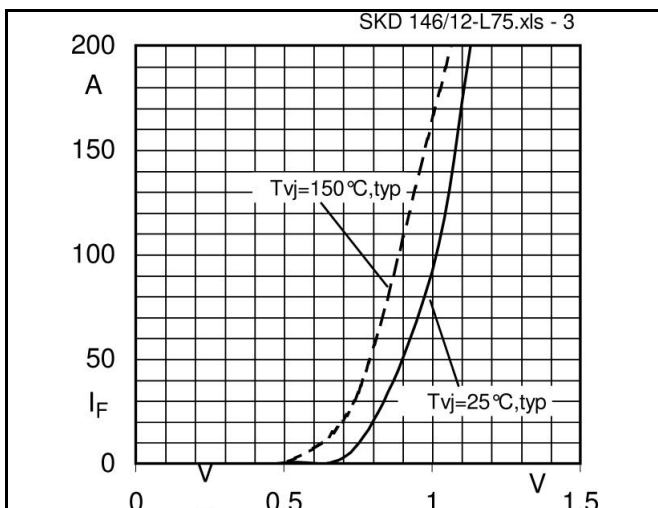
Fig. 3 Forward characteristic of a single rectifier diode
