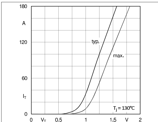
Fig. 7: On-state characteristics
