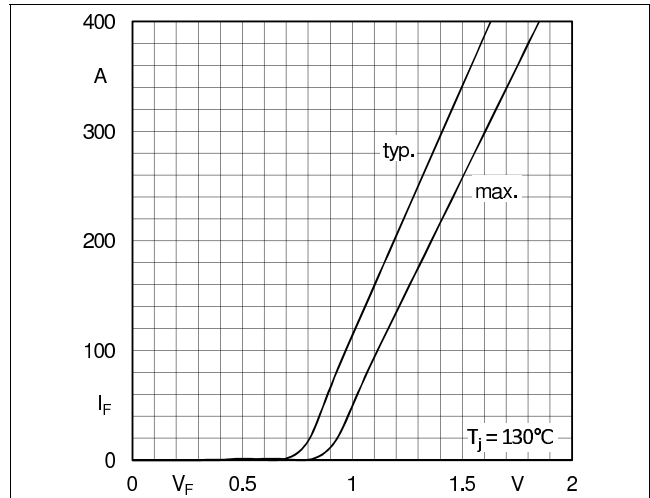
Fig. 15: Forward characteristics
