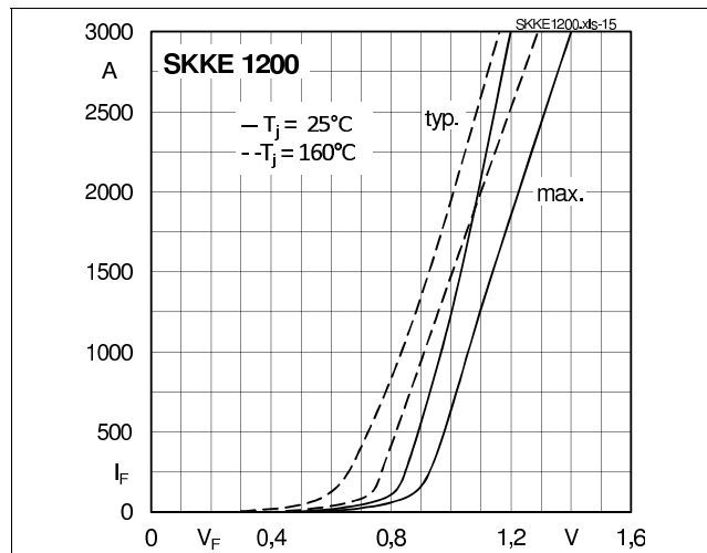
Fig. 15: Forward characteristics
