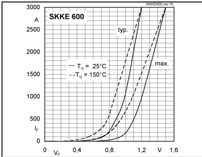
Fig. 15 Forward characteristics
