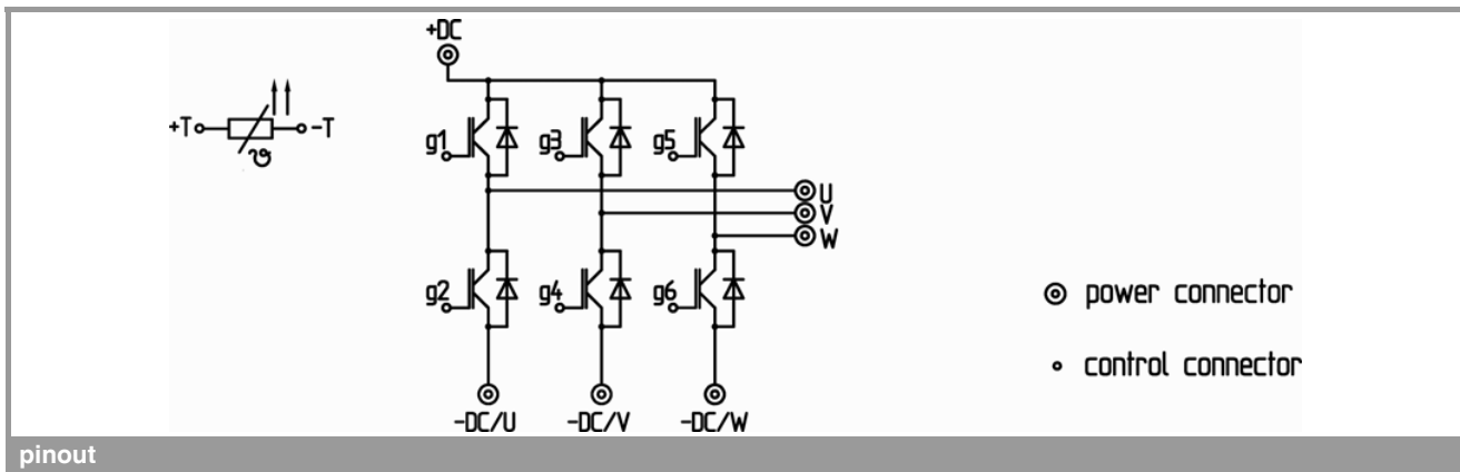
pinout, dimensions
