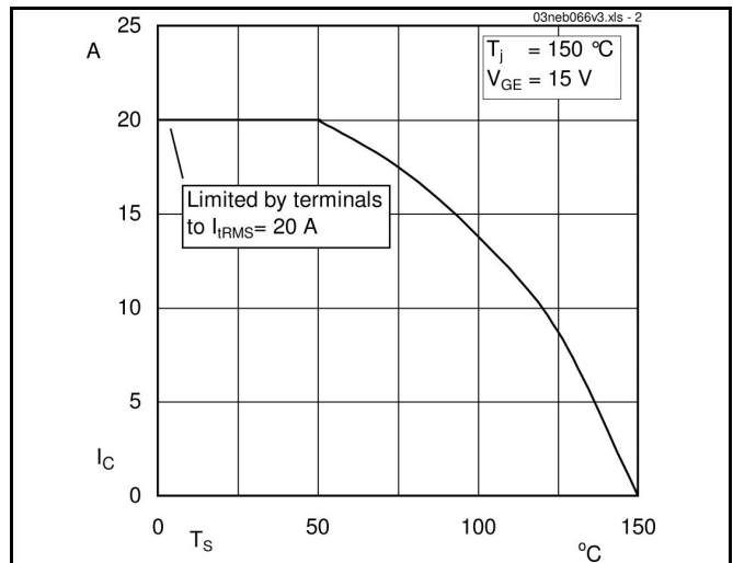
Fig. 2 Typ. rated output current
