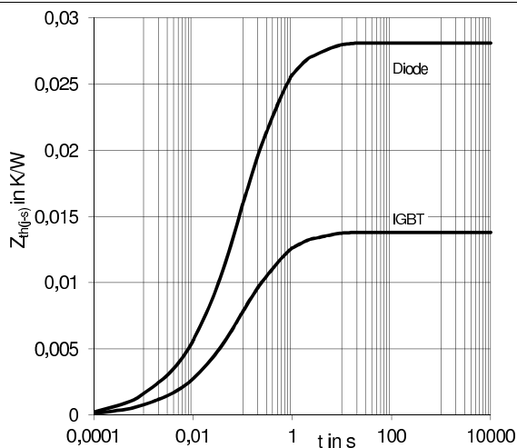
Fig. 5: Transient thermal impedance Z_{th}(j-s)
