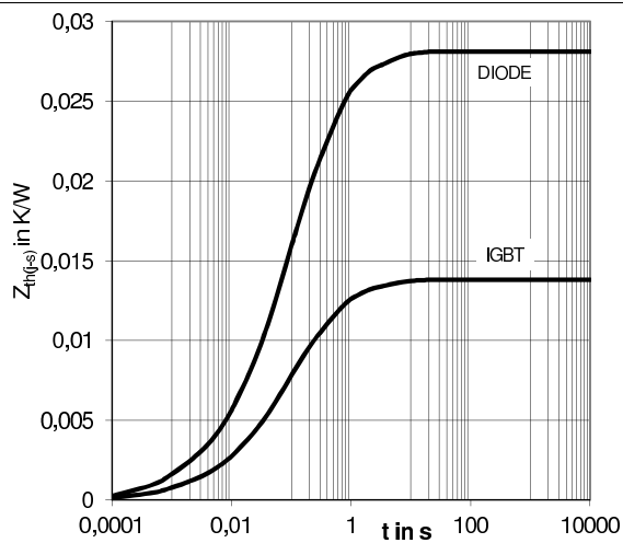
Fig. 5: Transient thermal impedance Z_{th}(j-s)
