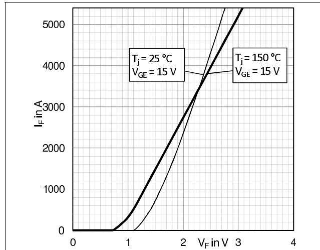
Fig. 2: Typical diode output characteristics
