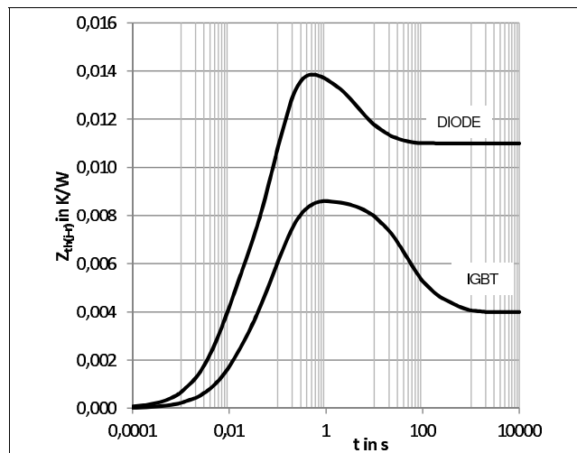
Fig. 6: Transient thermal impedance Z_{th}(j-r)
