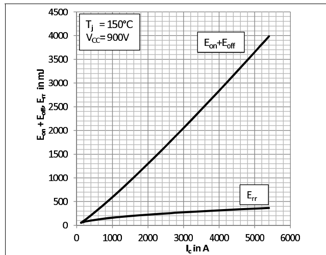
Fig. 4: Typical energy losses E = f(I_C, V_{CC}, T_j)
