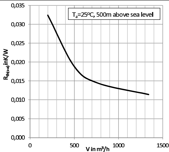
Fig. 9: Thermal resistance R_{th}(s-a) versus flow rate V
