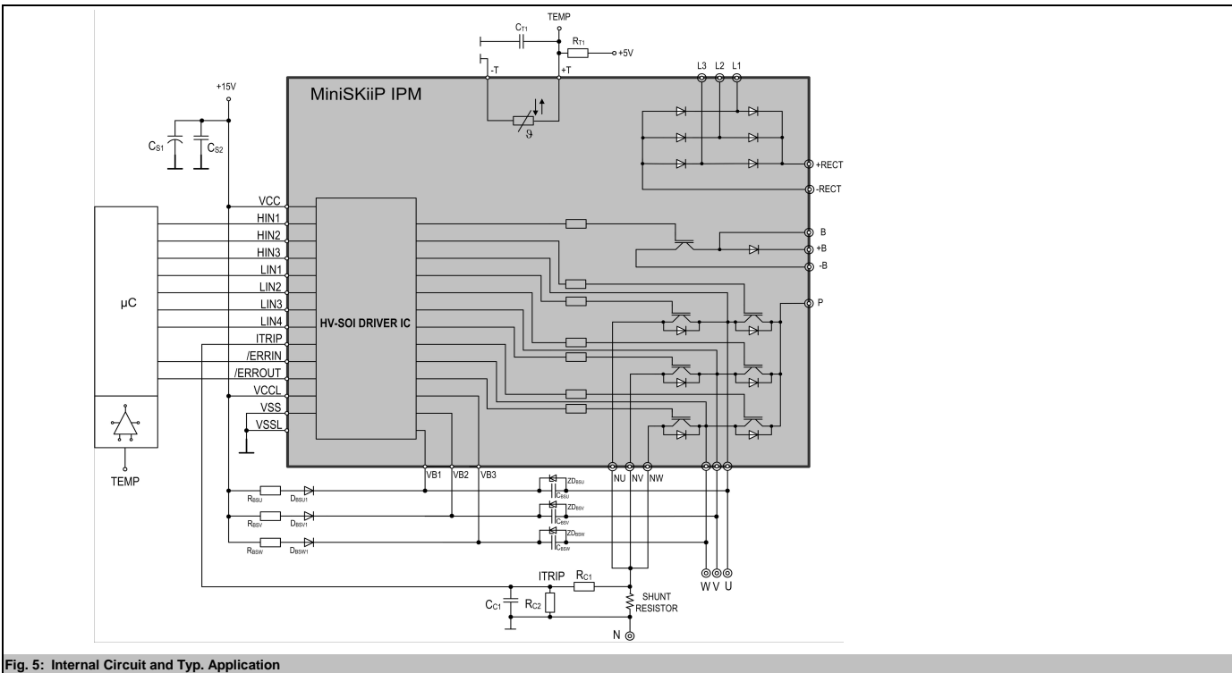
Fig. 5: Internal Circuit and Typ. Application
