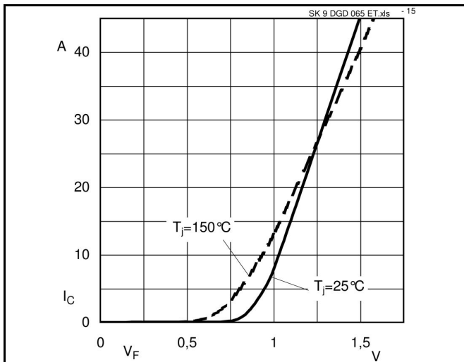
Fig. 15 Typ. Input Bridge Diode forward characteristic
