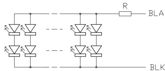
Backlight Circuit Scale=free
