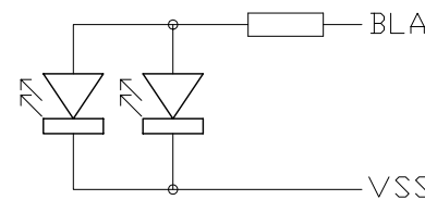
Backlight Circuit Scale=free
