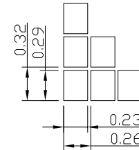
Pixel Details Scale=20/1
