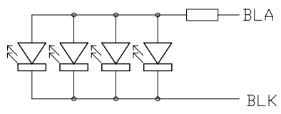
Backlight Circuit (No. of LEDs = 4pcs) Scale=free
