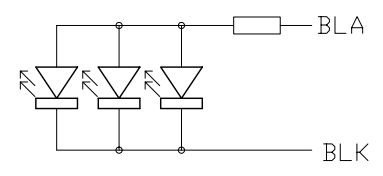
Backlight Circuit (No. of LEDs = 3pcs) Scale=free
