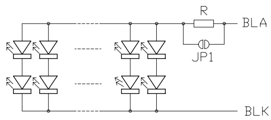
Backlight Circuit Scale=free
