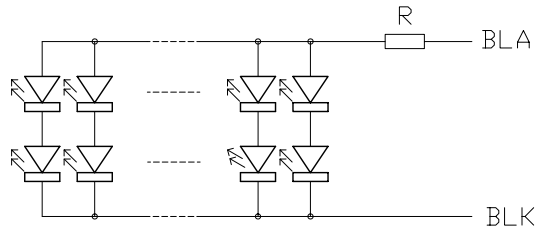
Backlight Circuit Scale=free
