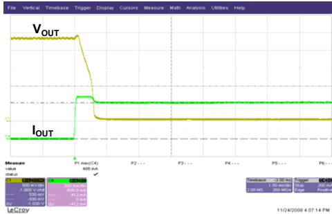
Current Limit ( V_{OUT} vs. I_{OUT} )
