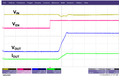
Enable ON Sequence ( R_L=16\Omega )
