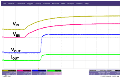
Power ON ( R_L=16\Omega )
