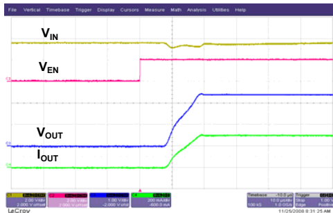
Enable ON Sequence ( R_L=8\Omega )
