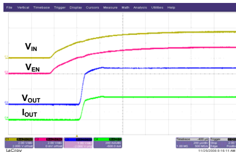
Power ON ( R_L=8\Omega )
