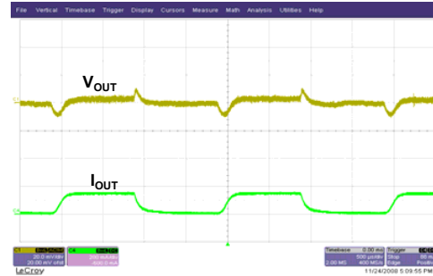
Load Transient I_{OUT}=0mA \sim 150mA
