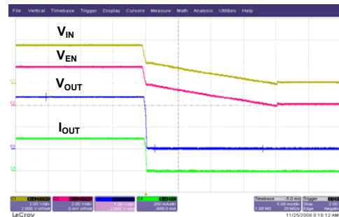
Power OFF ( R_L=8\Omega )
