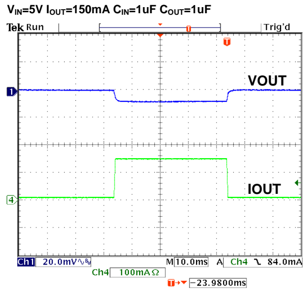
Figure 11. Load Transient Response
