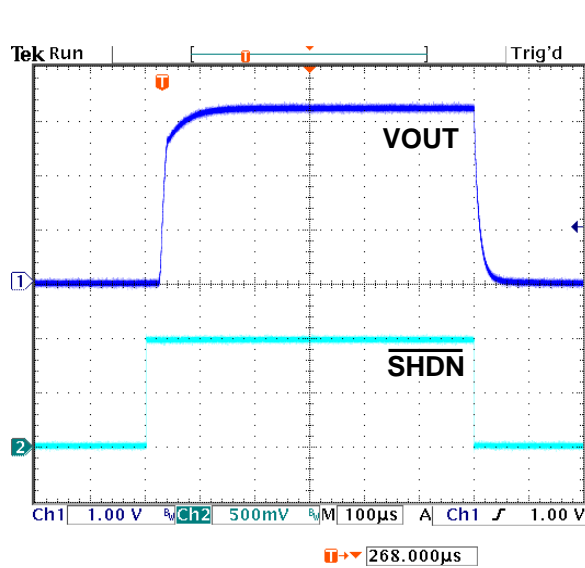
Figure 10. Shutdown Function
