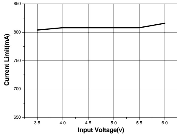
Figure 5. Current limit vs. Input Voltage
