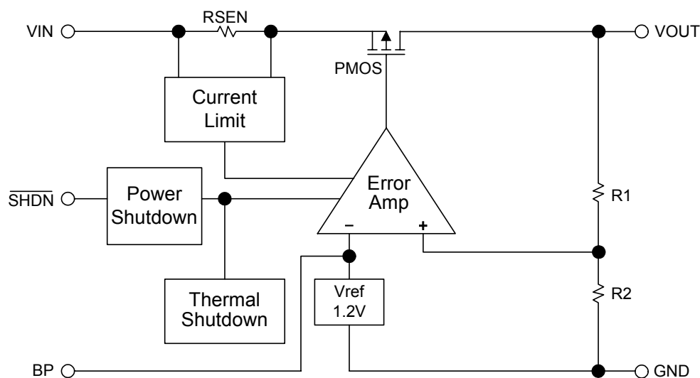
Figure 3. Block Diagram of APE8805A
