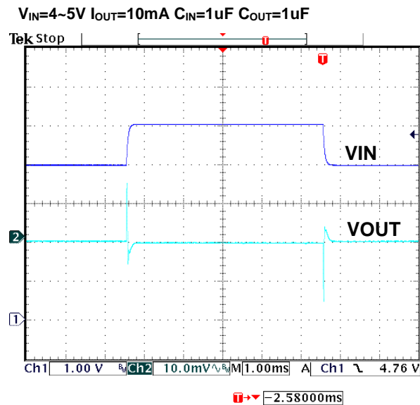
Figure 12. Line Transient Response
