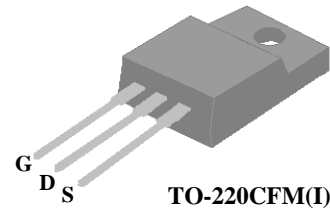
TO-220CFM(I)
