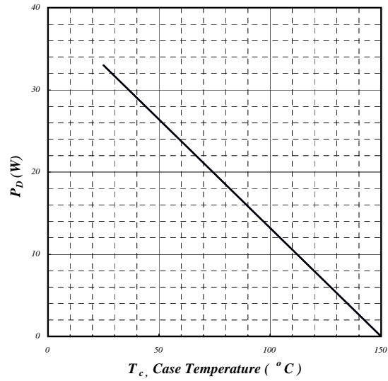
Fig 6. Typical Power Dissipation
