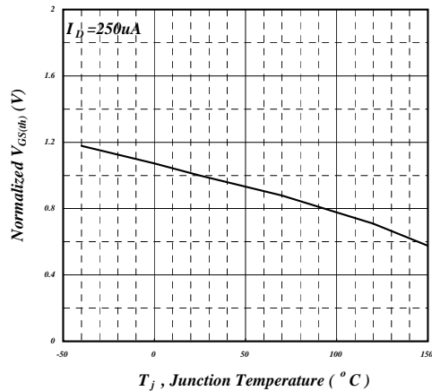
Fig 6. Gate Thrs. Junction Temperature
