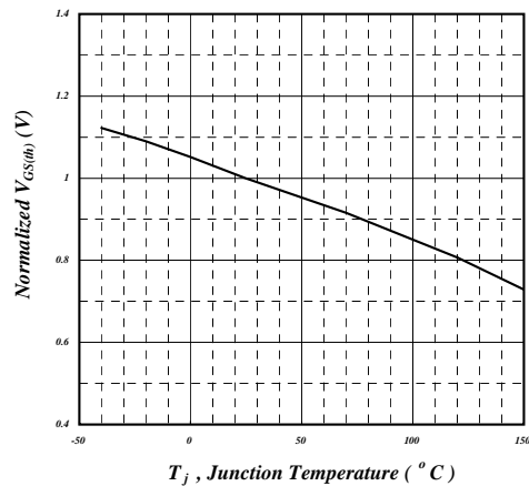
Fig 6. Gate Ths.v.s. Junction Temperature
