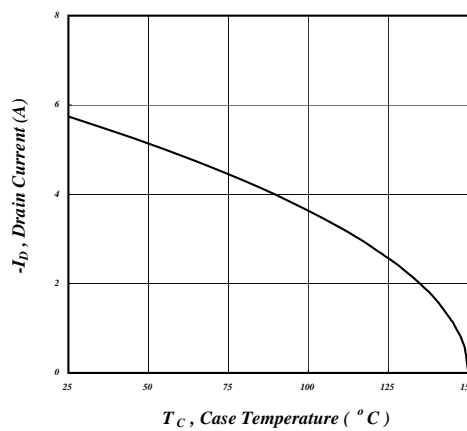
Fig 12. Maximum Continuous Drain Current v.s. Case Temperature
