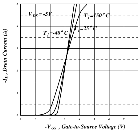
Fig 11. Transfer Characteristics
